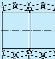
With Pin Type Cages Figure 2
